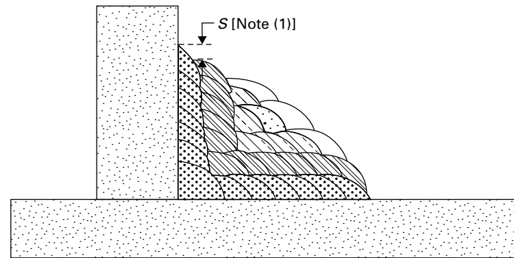
Typical Fillet Weld
