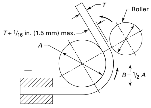
Figure QB-466.3 Guided-Bend Wrap Around Jig
