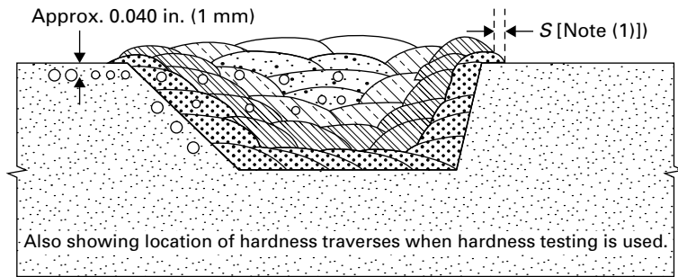
Completed Partial-Penetration Weld
