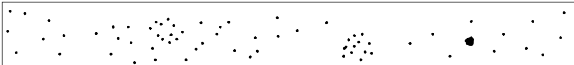
Typical Quantity and Size Permitted in 6 in. (150 mm) Length of Weld Over 1/2 in. (13 mm) to 1 in. (25 mm) Thickness
