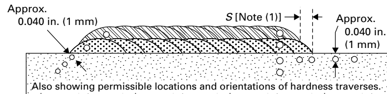
Overlay Weld
